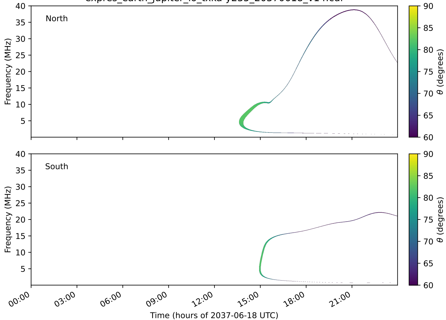
expres_earth_jupiter_io_txka-y235_20370618_v14.cdf
