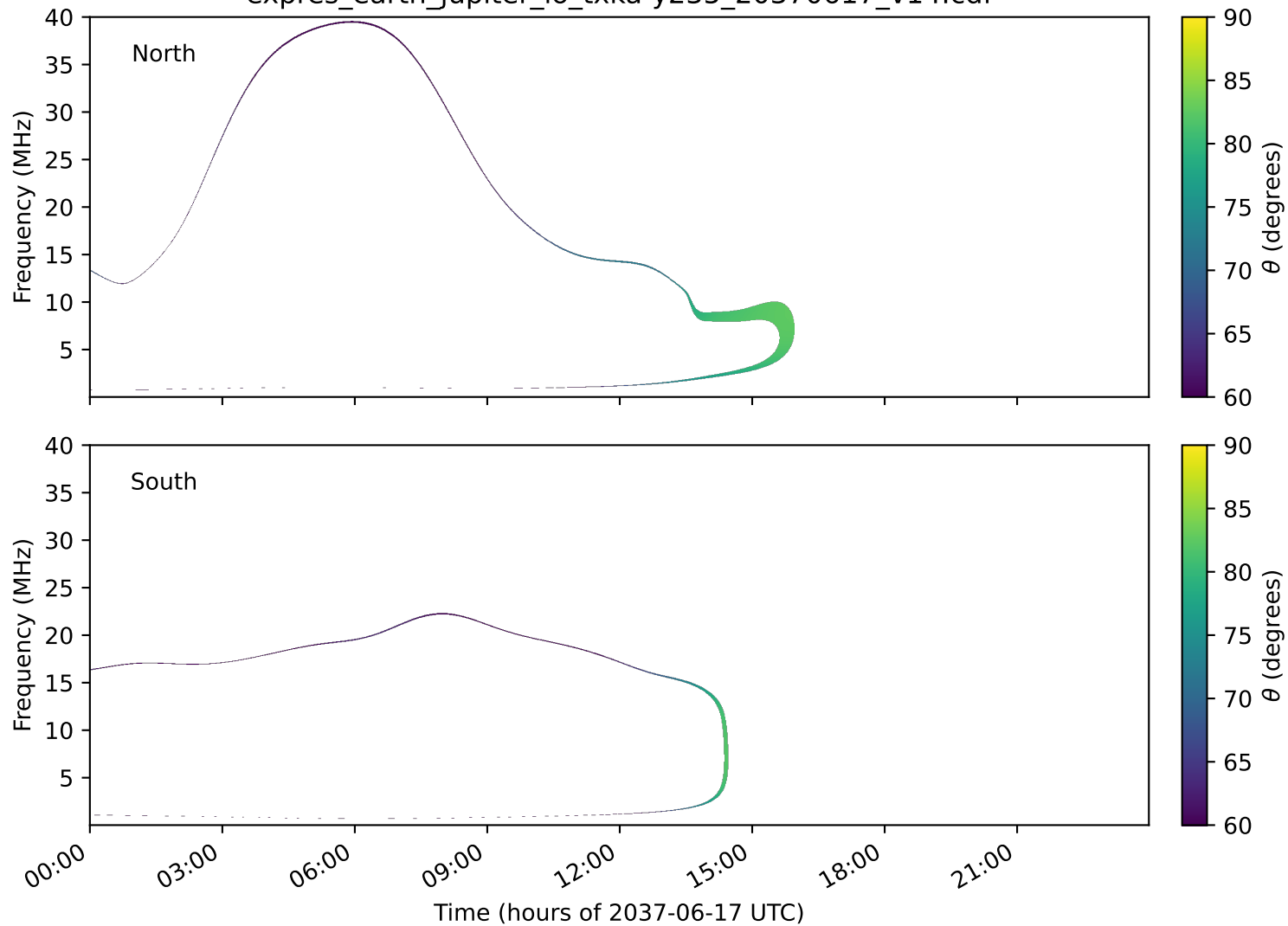
expres_earth_jupiter_io_txka-y235_20370617_v14.cdf
