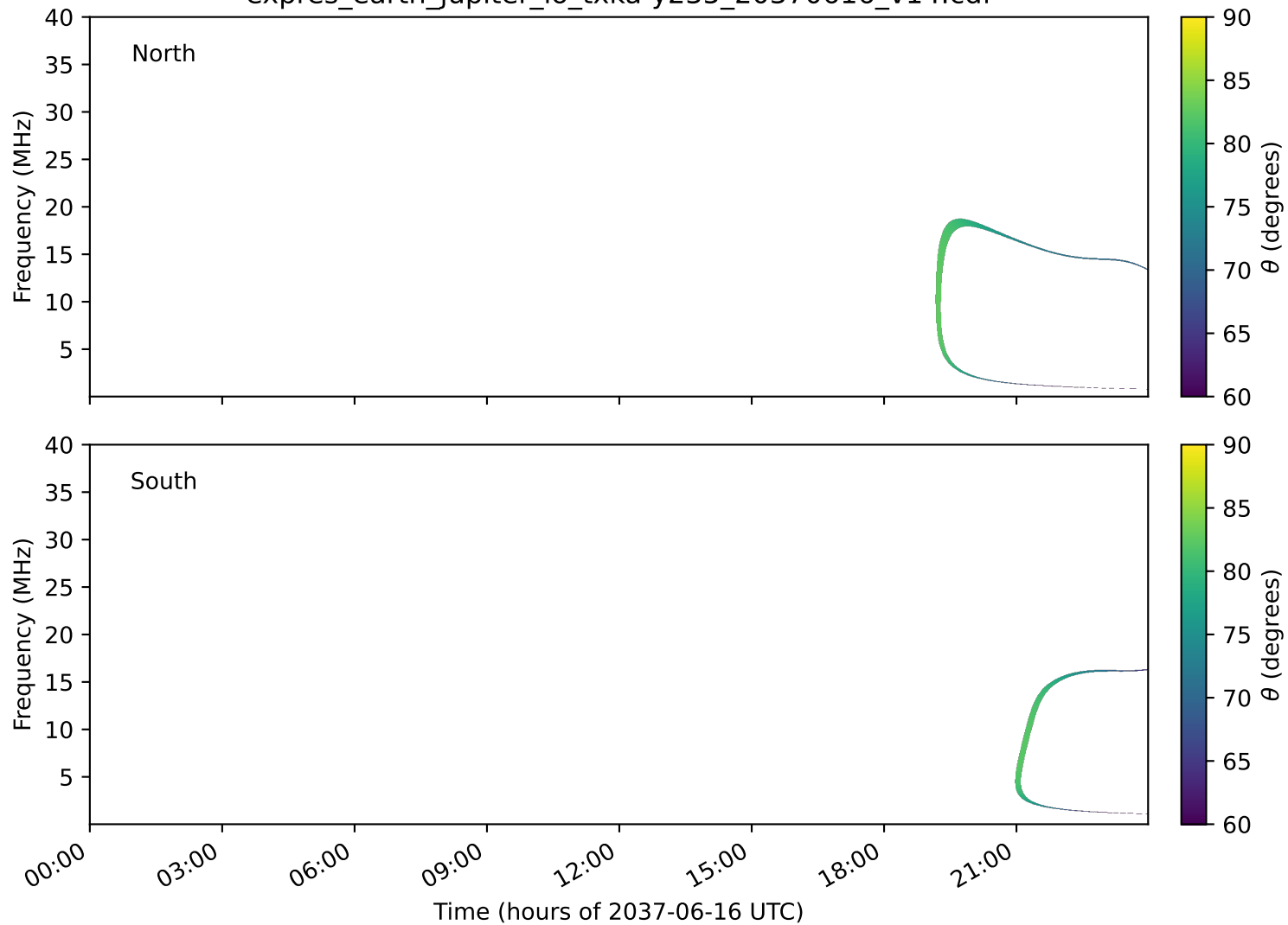
expres_earth_jupiter_io_txka-y235_20370616_v14.cdf
