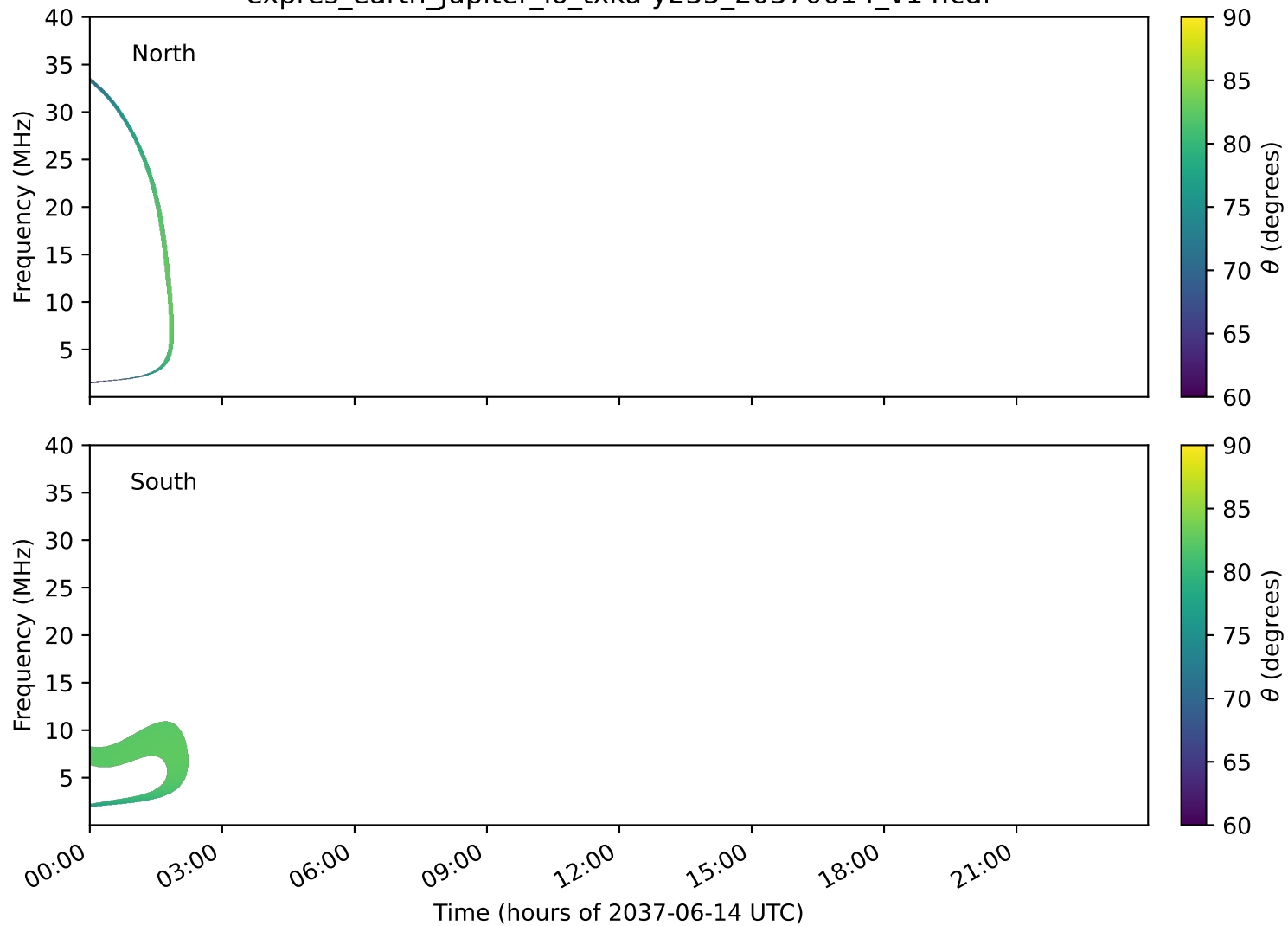
expres_earth_jupiter_io_txka-y235_20370614_v14.cdf
