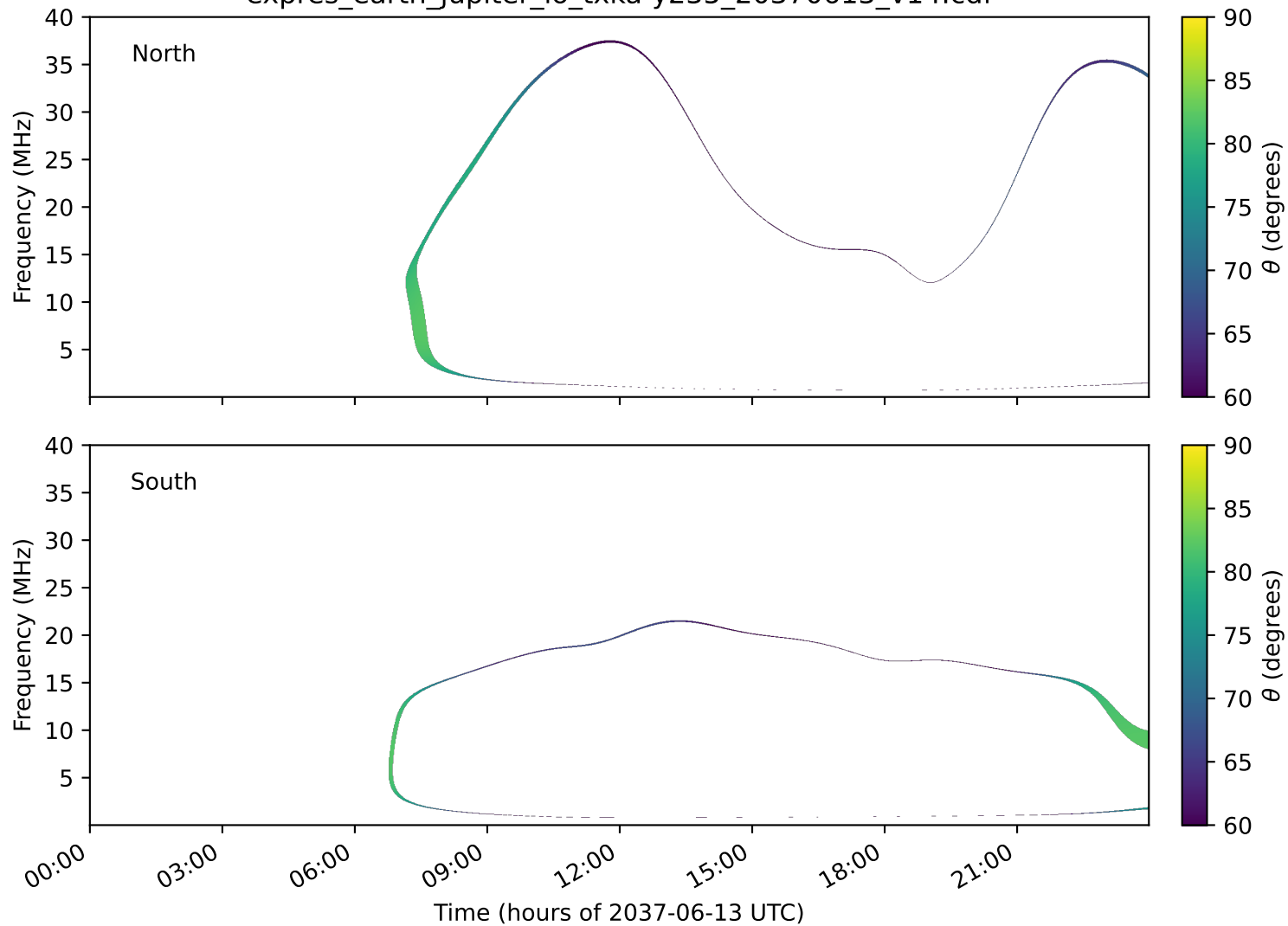
expres_earth_jupiter_io_txka-y235_20370613_v14.cdf
