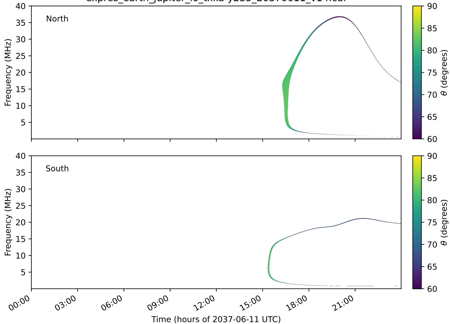
expres_earth_jupiter_io_txka-y235_20370611_v14.cdf
