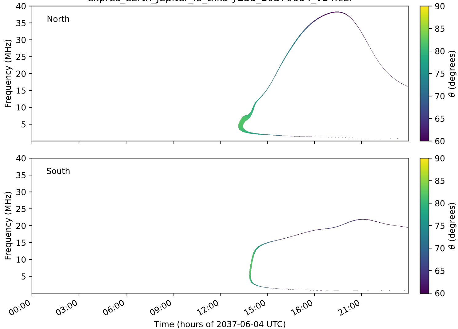
expres_earth_jupiter_io_txka-y235_20370604_v14.cdf
