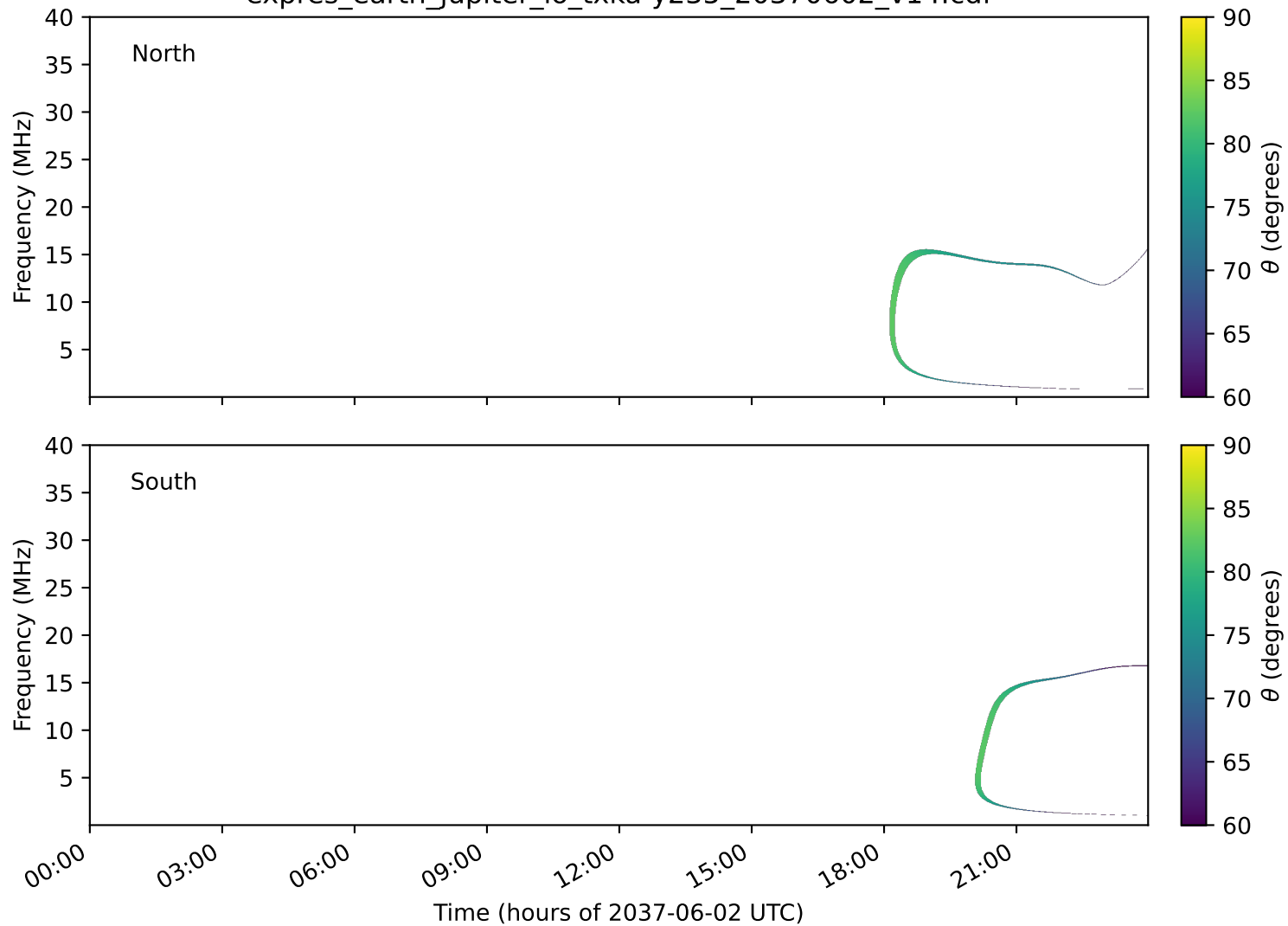
expres_earth_jupiter_io_txka-y235_20370602_v14.cdf
