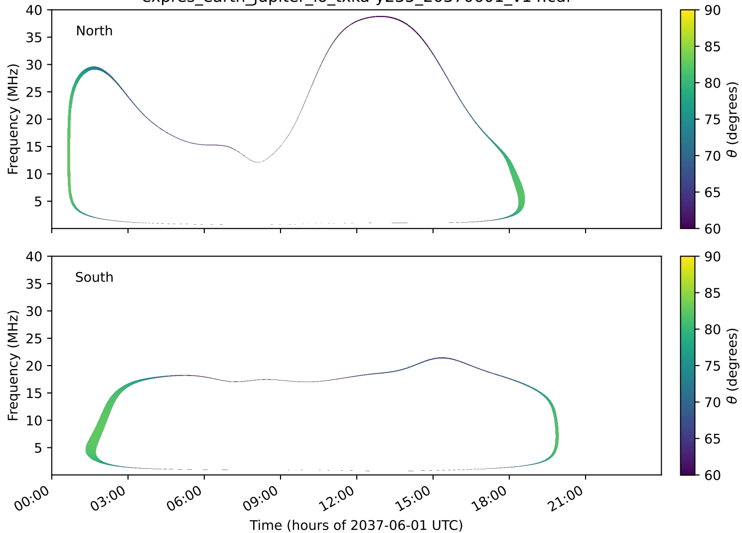
expres_earth_jupiter_io_txka-y235_20370601_v14.cdf
