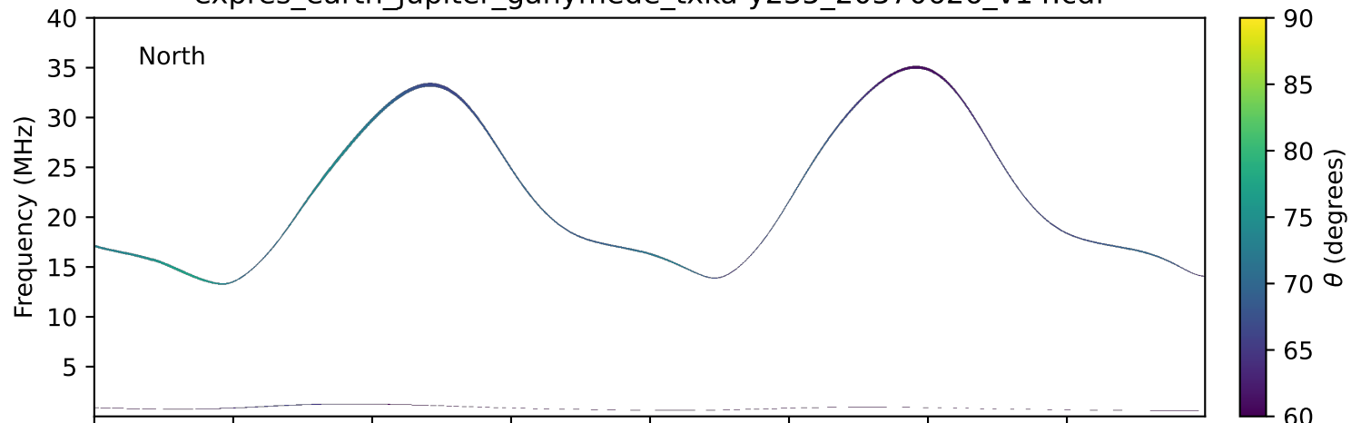
expres_earth_jupiter_ganymede_txka-y235_20370626_v14.cdf
