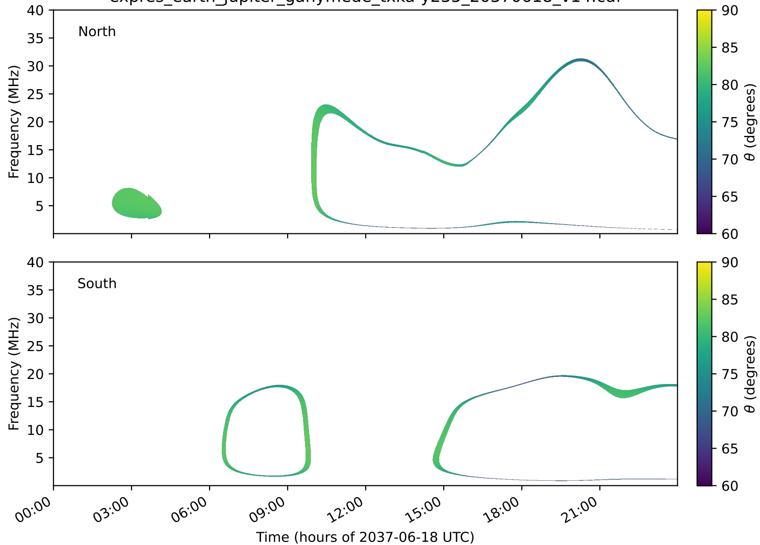
expres_earth_jupiter_ganymede_txka-y235_20370618_v14.cdf
