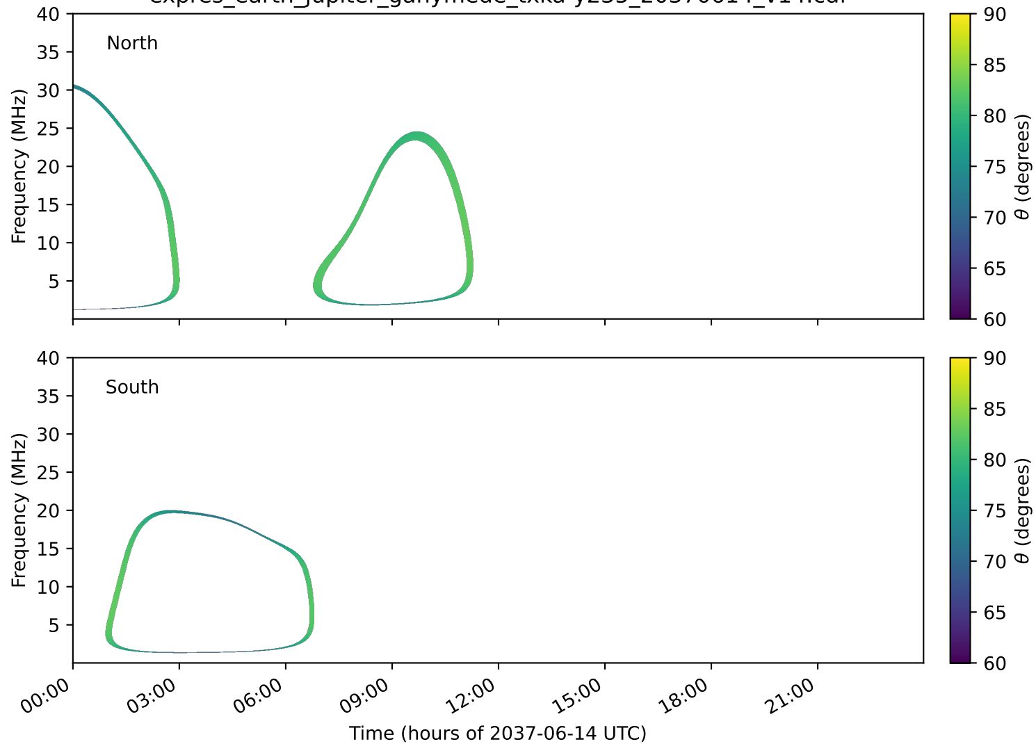
expres_earth_jupiter_ganymede_txka-y235_20370614_v14.cdf
