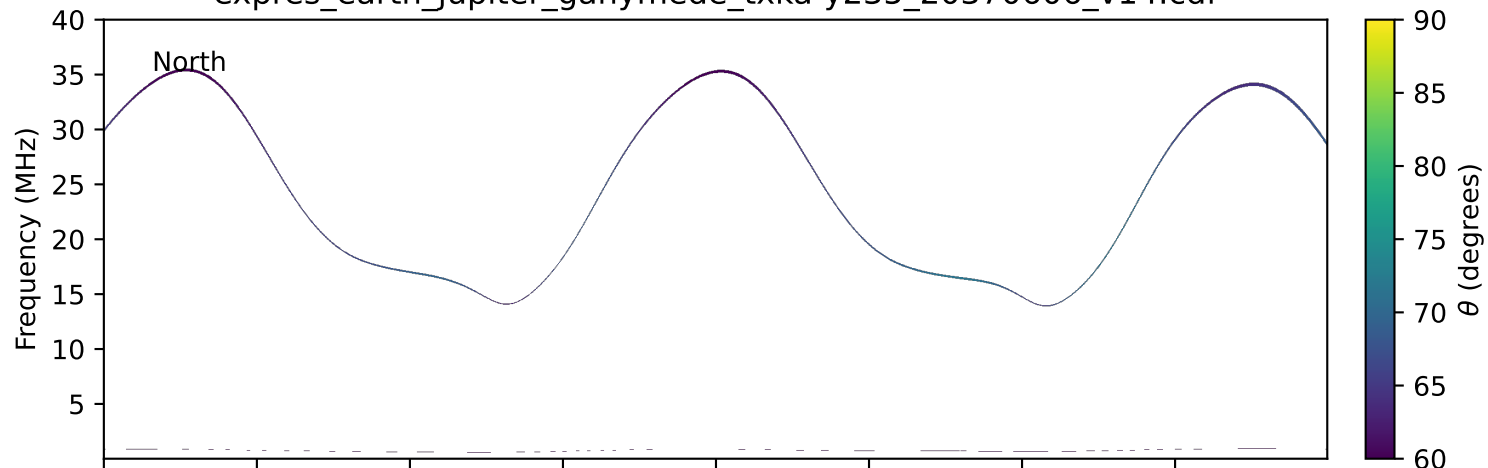
expres_earth_jupiter_ganymede_txka-y235_20370606_v14.cdf
