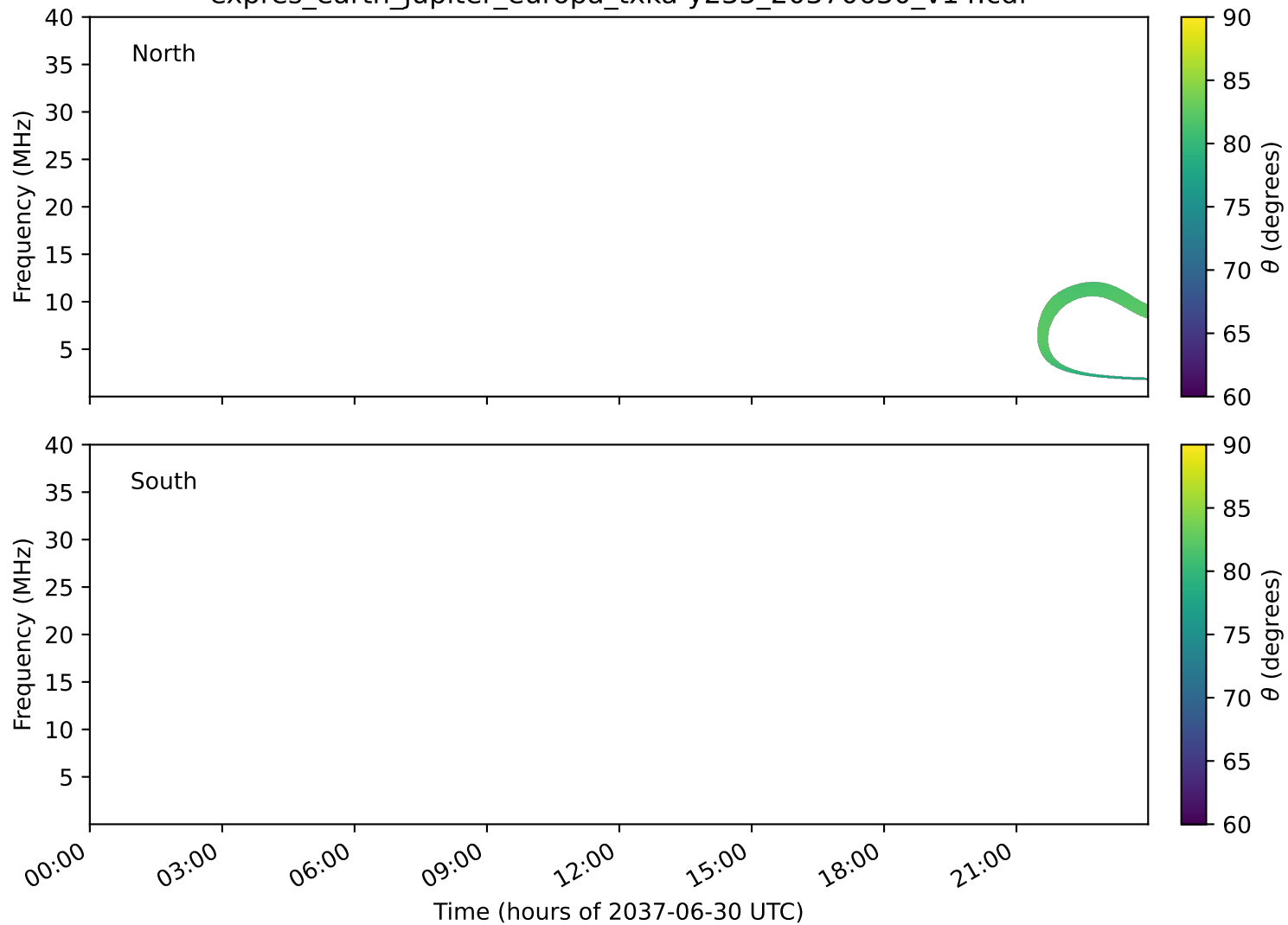
expres_earth_jupiter_europa_txka-y235_20370630_v14.cdf
