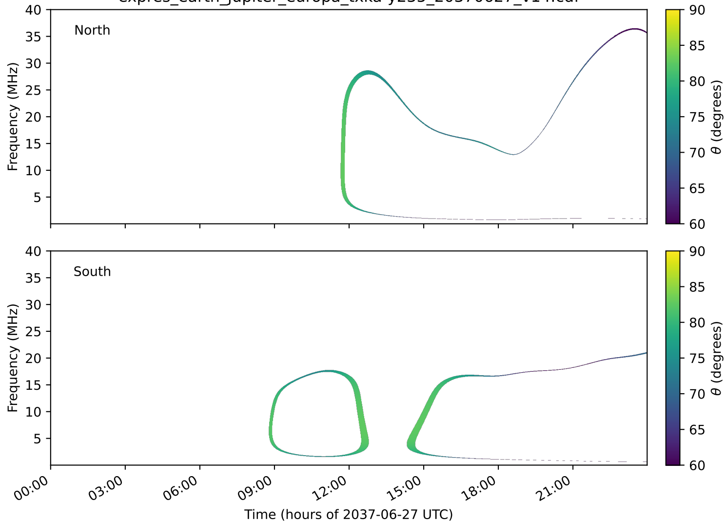
expres_earth_jupiter_europa_txka-y235_20370627_v14.cdf
