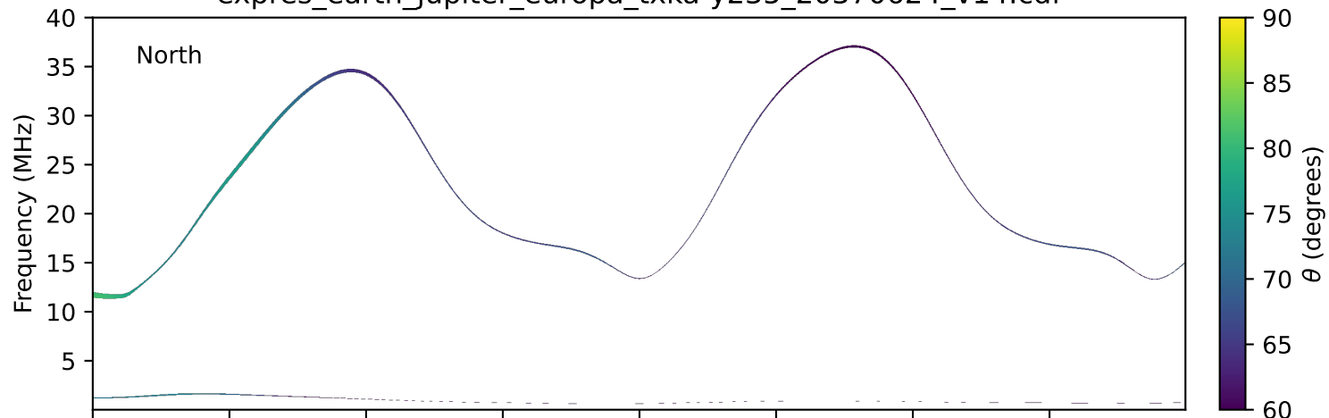
expres_earth_jupiter_europa_txka-y235_20370624_v14.cdf
