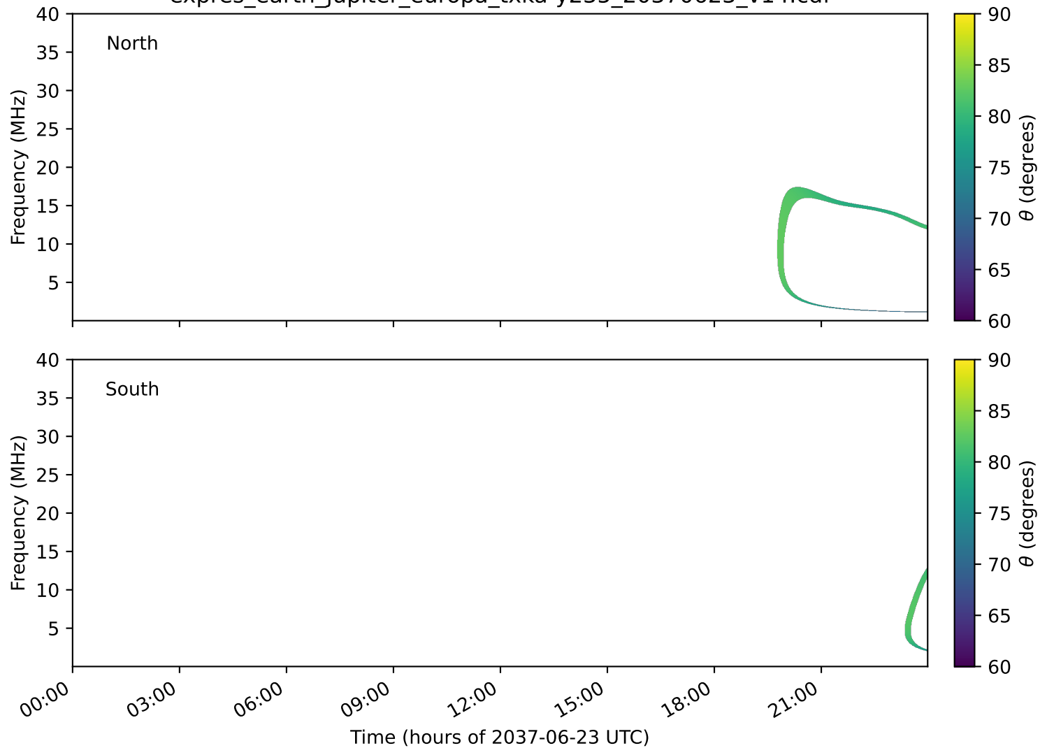
expres_earth_jupiter_europa_txka-y235_20370623_v14.cdf
