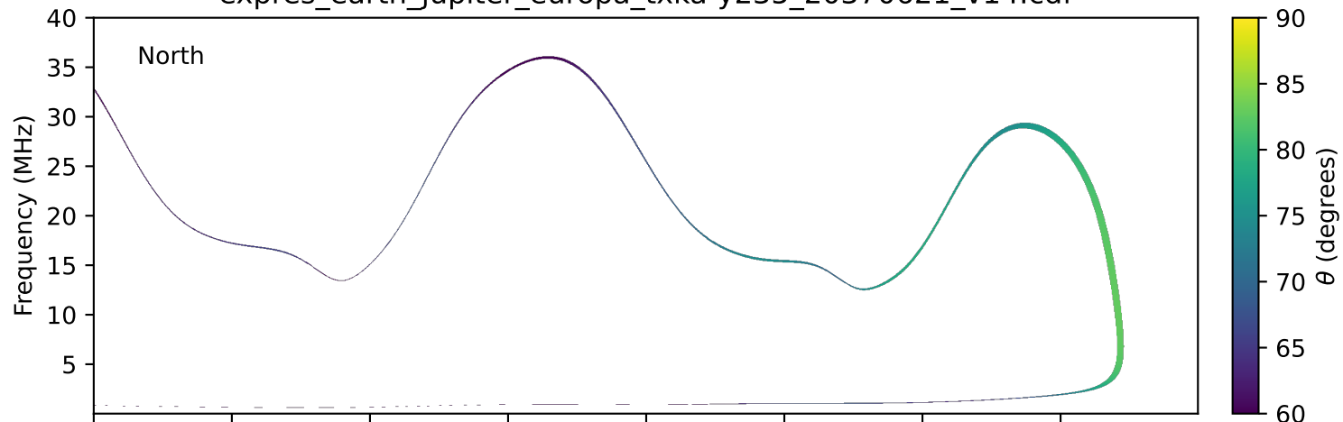
expres_earth_jupiter_europa_txka-y235_20370621_v14.cdf
