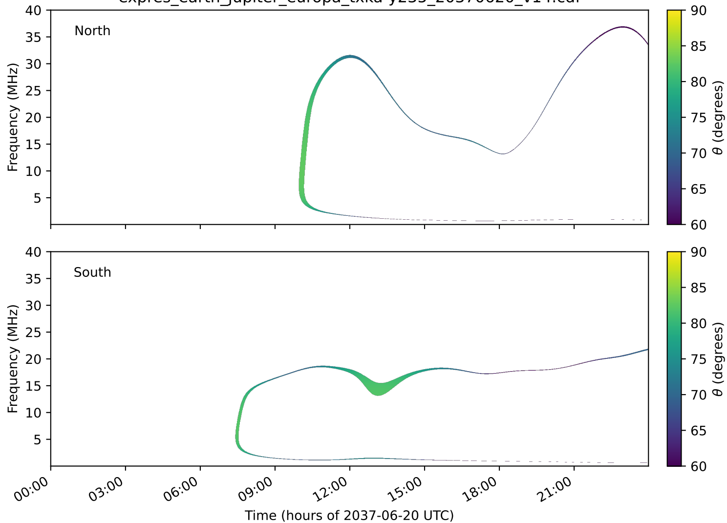
expres_earth_jupiter_europa_txka-y235_20370620_v14.cdf
