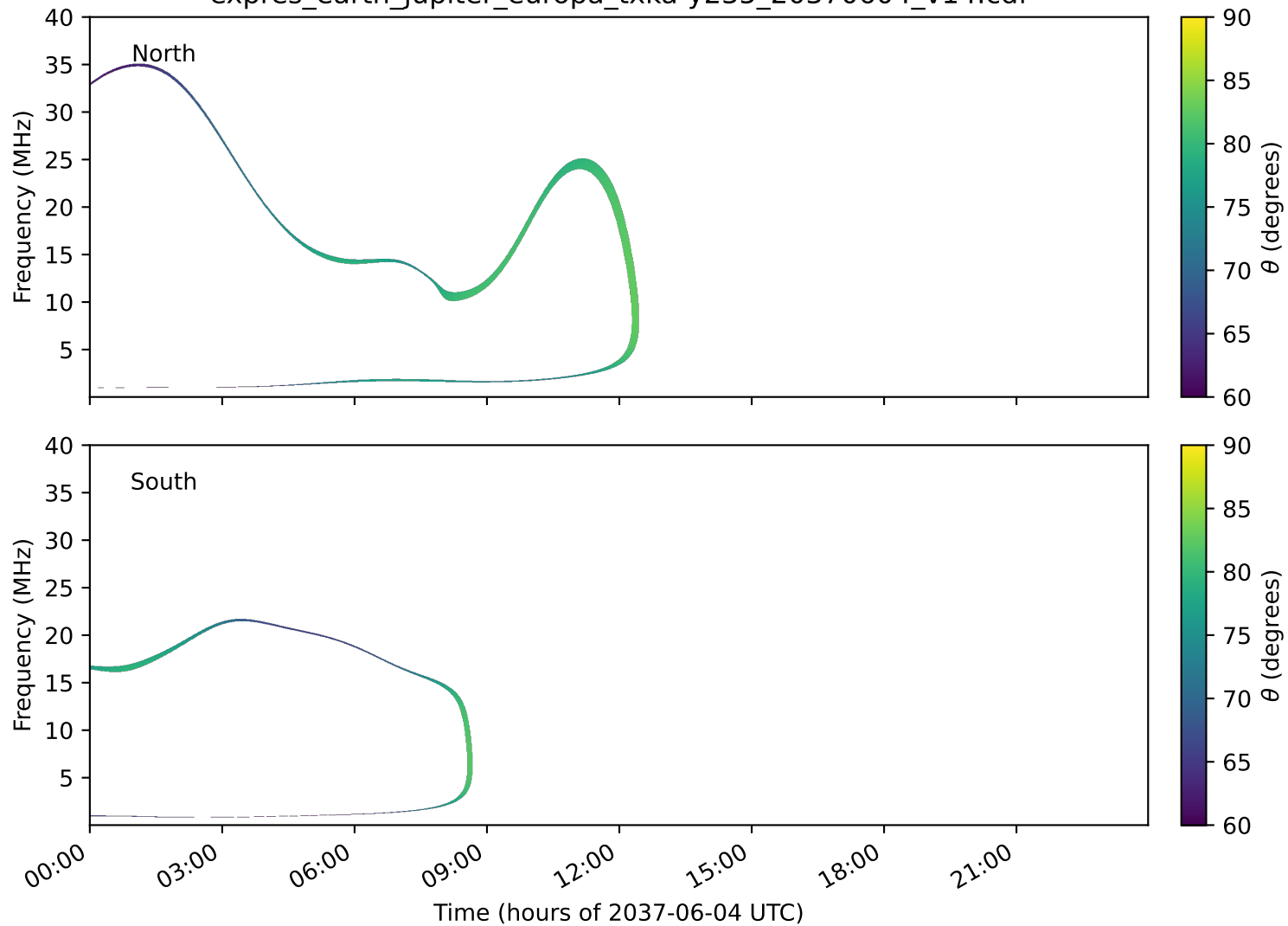
expres_earth_jupiter_europa_txka-y235_20370604_v14.cdf
