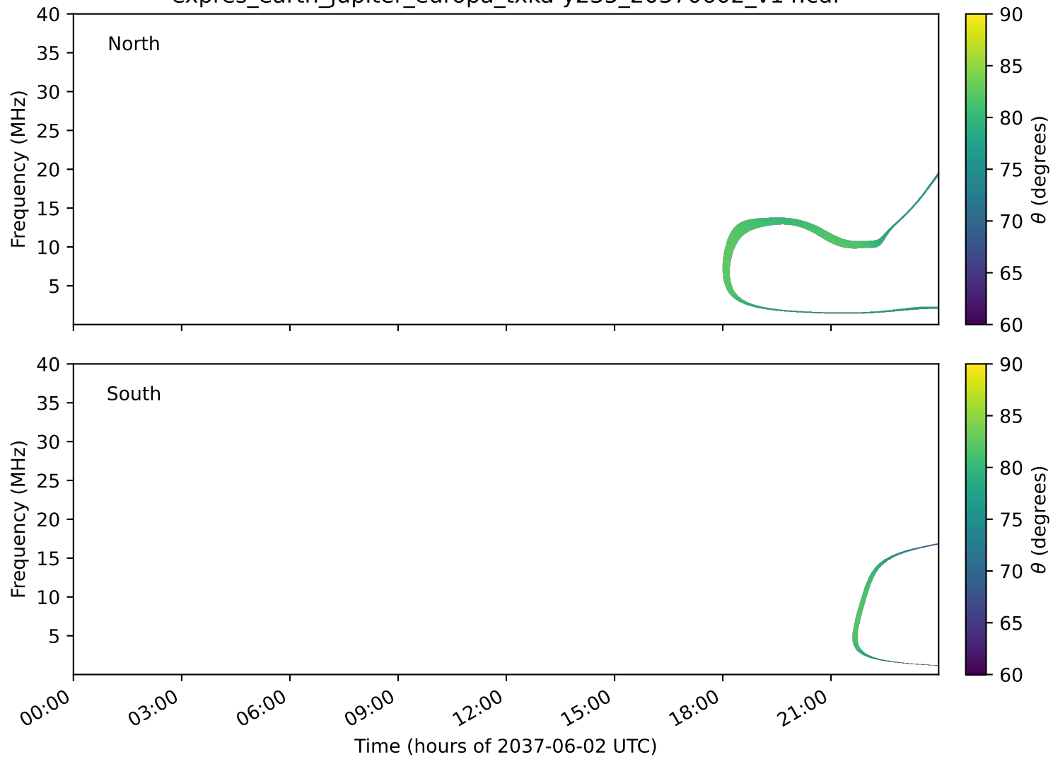
expres_earth_jupiter_europa_txka-y235_20370602_v14.cdf
