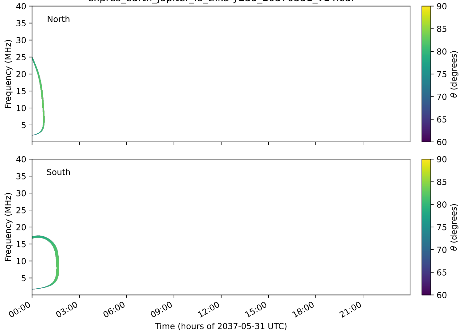
expres_earth_jupiter_io_txka-y235_20370531_v14.cdf
