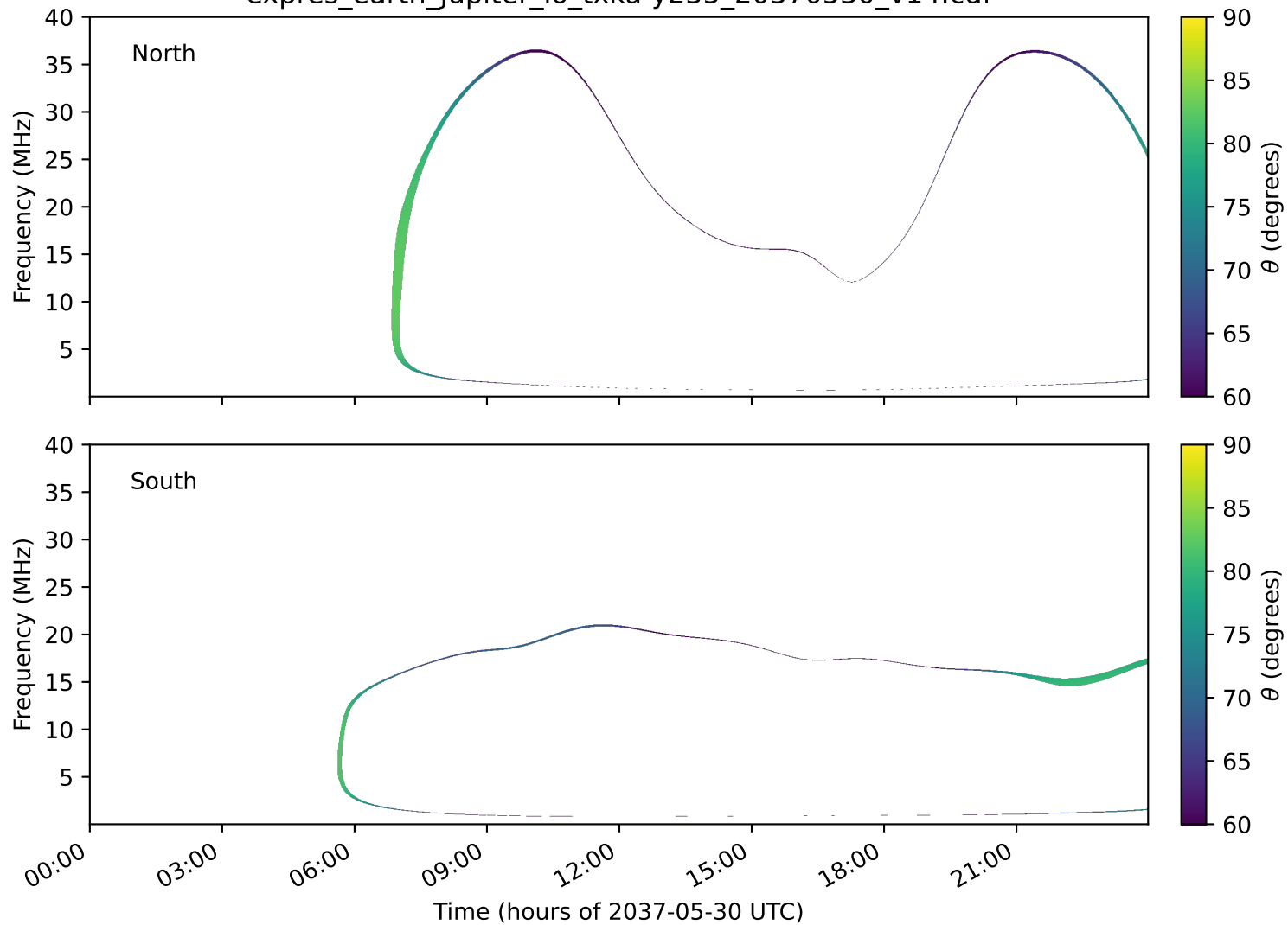
expres_earth_jupiter_io_txka-y235_20370530_v14.cdf
