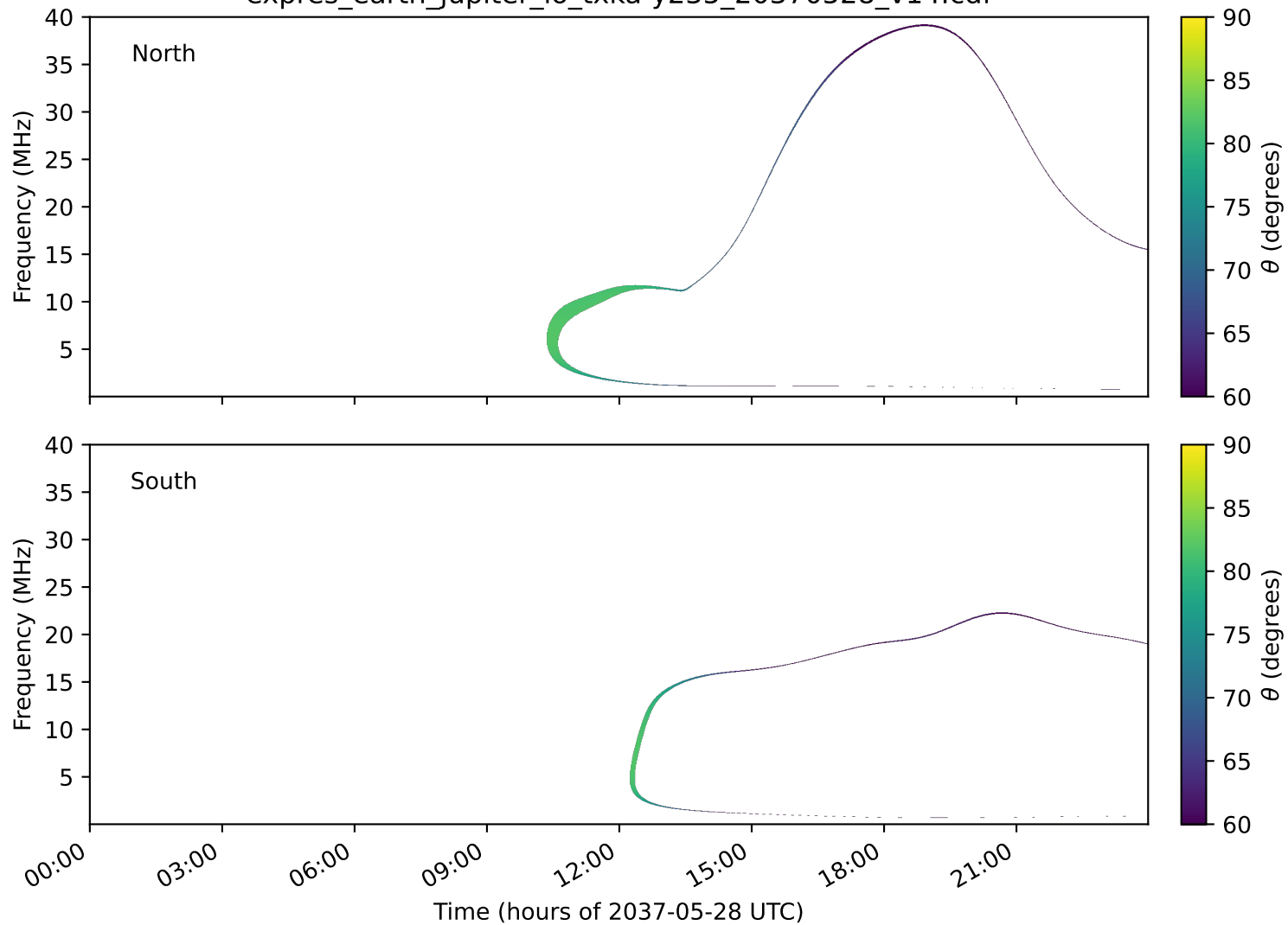
expres_earth_jupiter_io_txka-y235_20370528_v14.cdf
