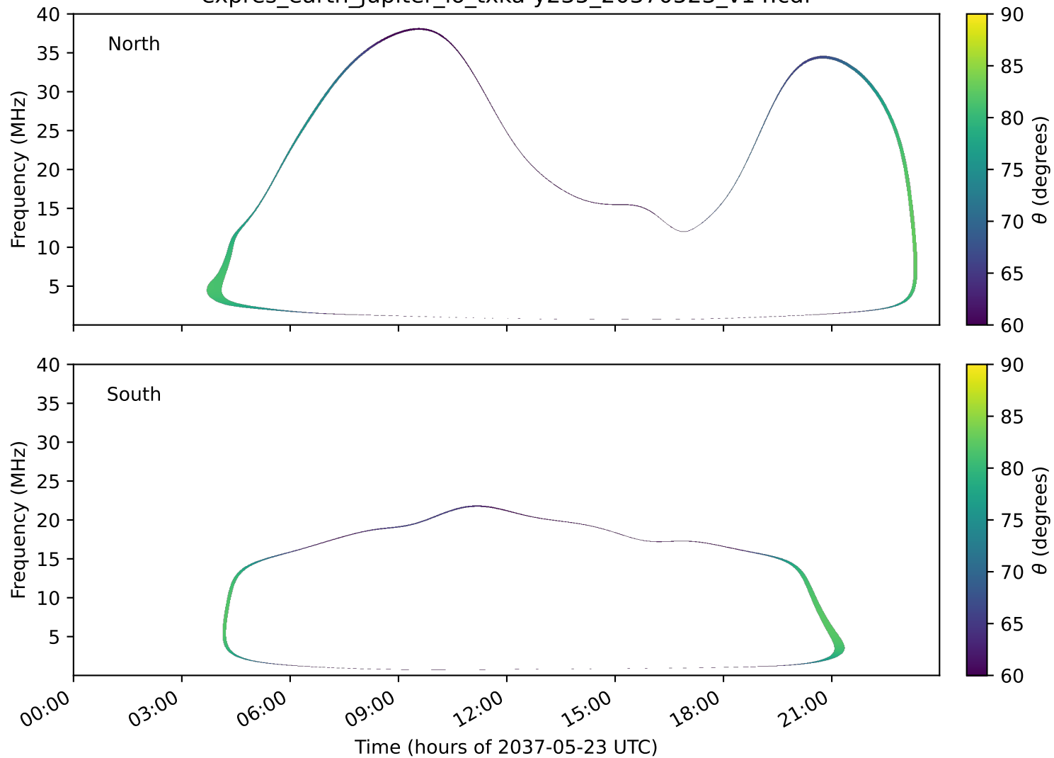
expres_earth_jupiter_io_txka-y235_20370523_v14.cdf
