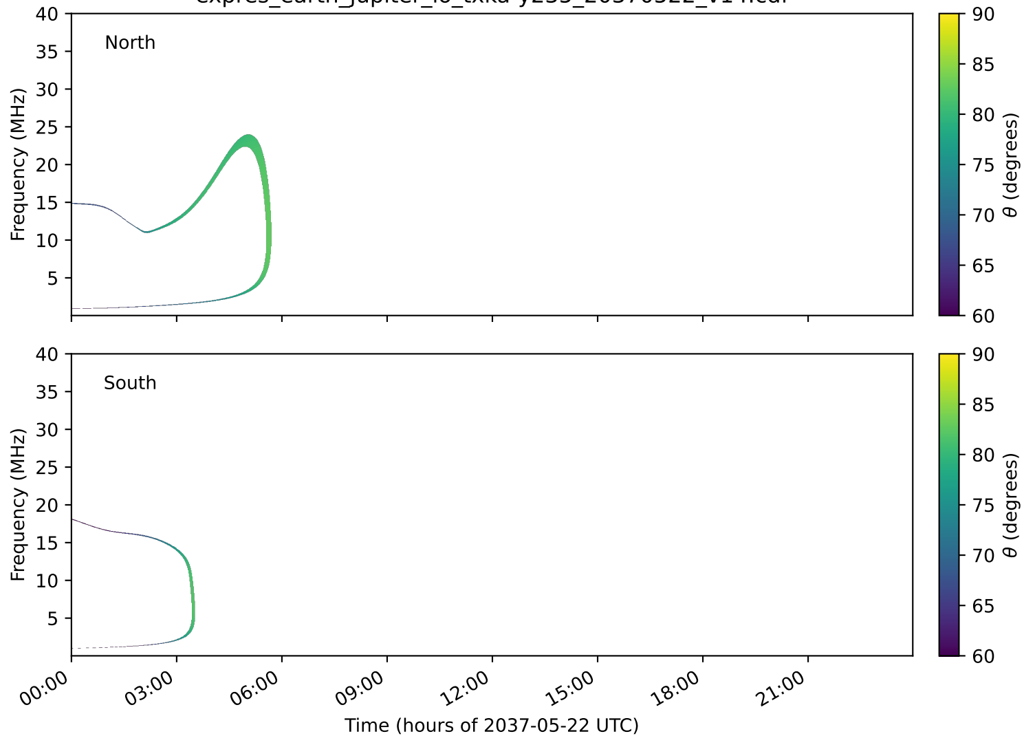
expres_earth_jupiter_io_txka-y235_20370522_v14.cdf
