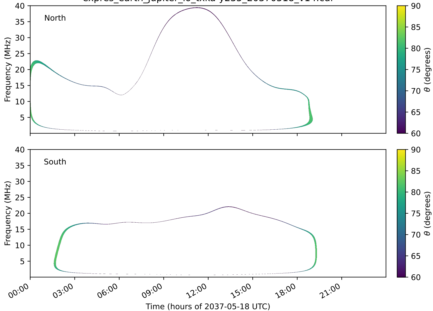
expres_earth_jupiter_io_txka-y235_20370518_v14.cdf
