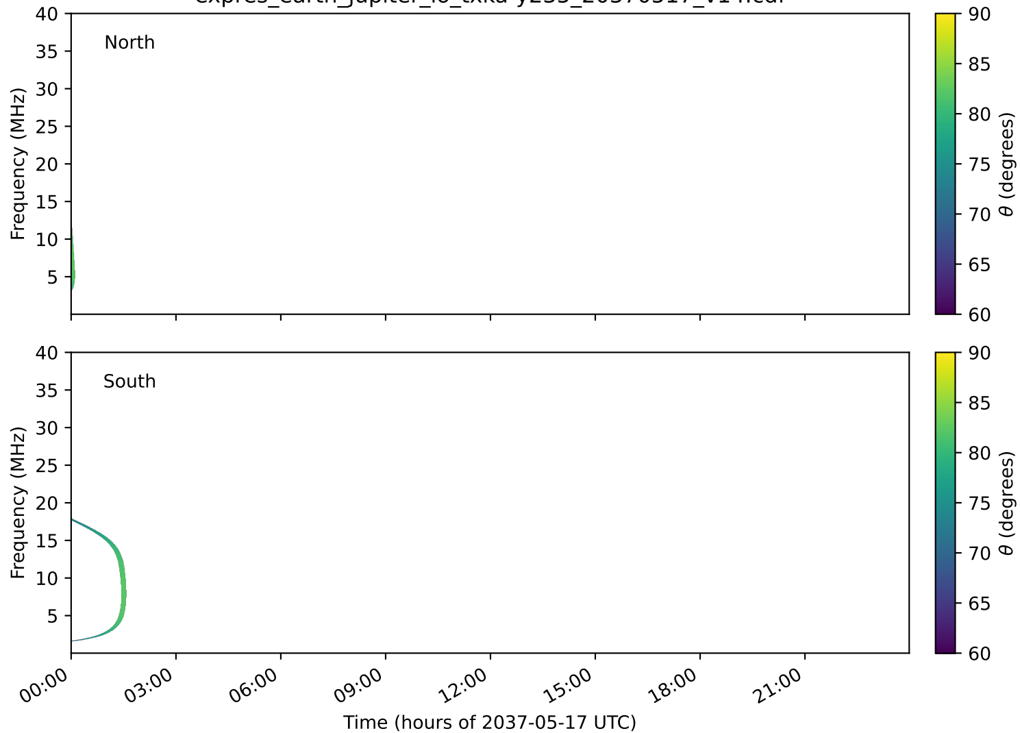
expres_earth_jupiter_io_txka-y235_20370517_v14.cdf
