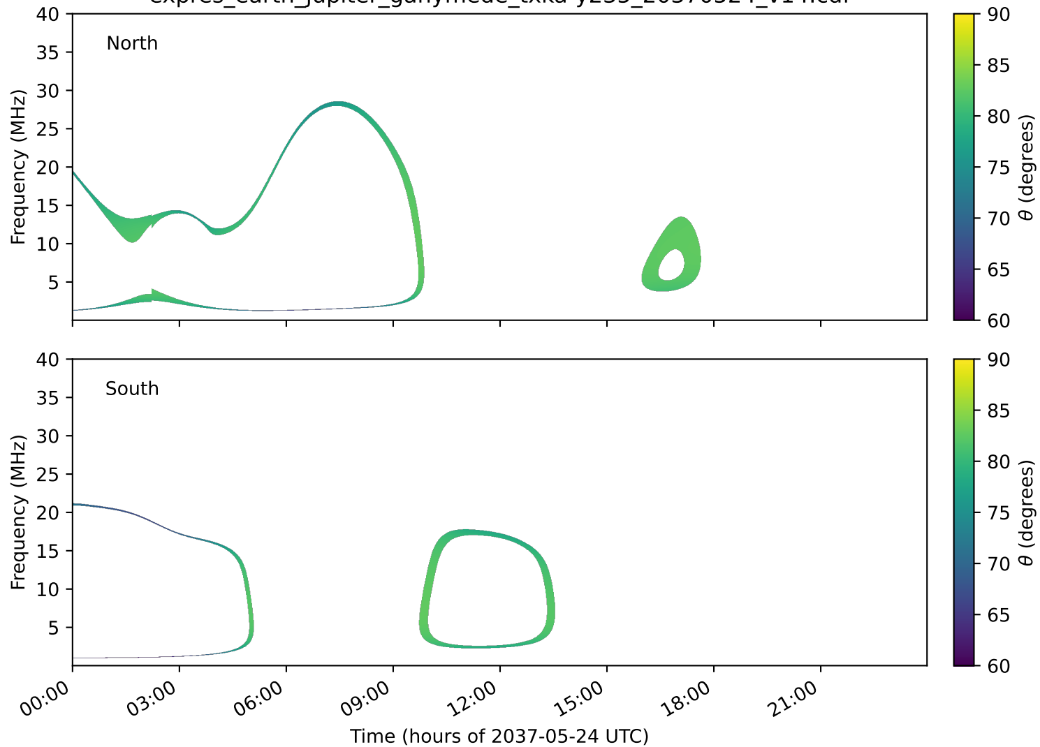
expres_earth_jupiter_ganymede_txka-y235_20370524_v14.cdf
