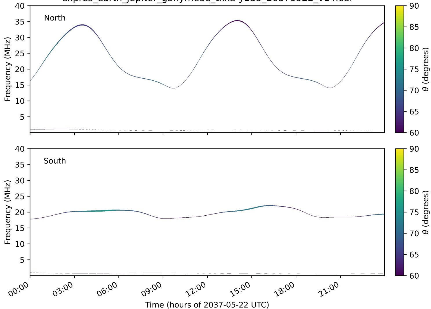
expres_earth_jupiter_ganymede_txka-y235_20370522_v14.cdf
