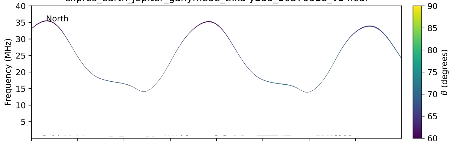
expres_earth_jupiter_ganymede_txka-y235_20370518_v14.cdf
