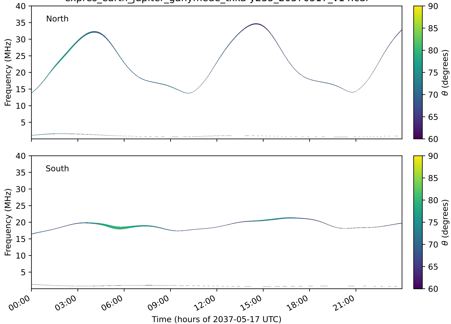
expres_earth_jupiter_ganymede_txka-y235_20370517_v14.cdf
