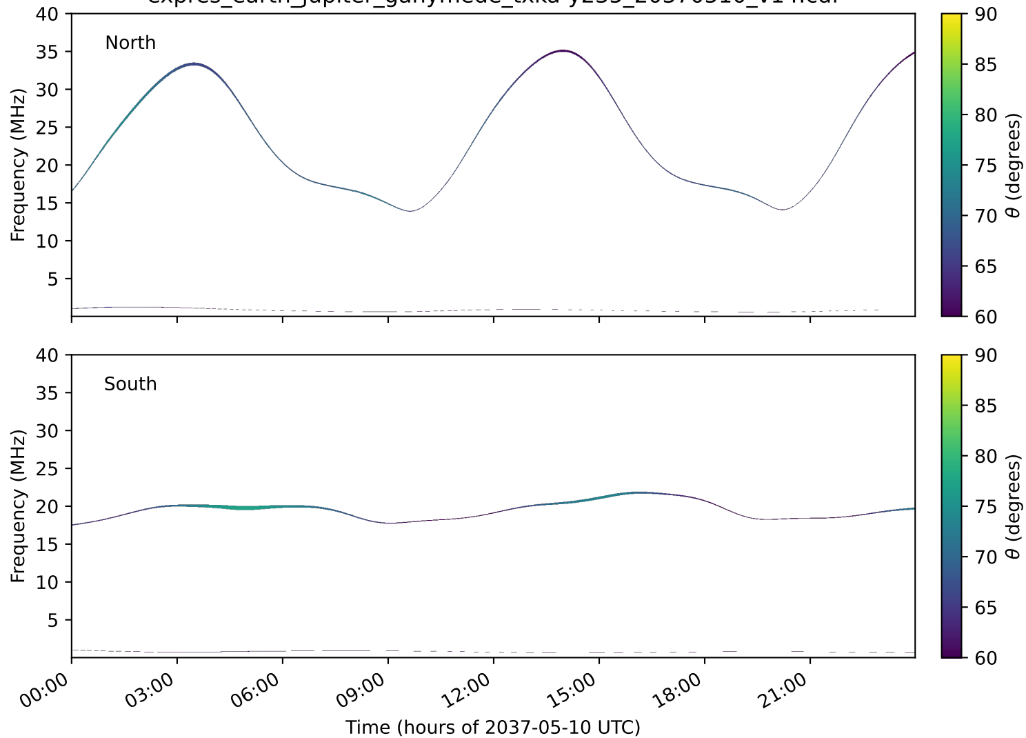
expres_earth_jupiter_ganymede_txka-y235_20370510_v14.cdf
