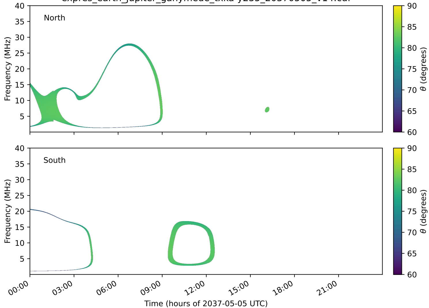
expres_earth_jupiter_ganymede_txka-y235_20370505_v14.cdf
