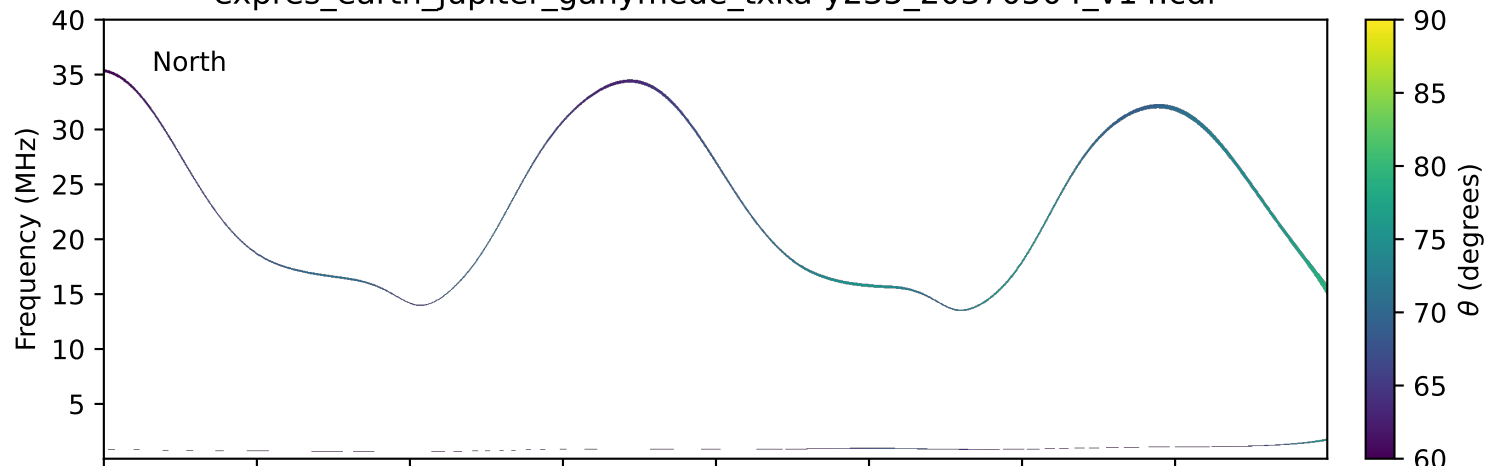
expres_earth_jupiter_ganymede_txka-y235_20370504_v14.cdf
