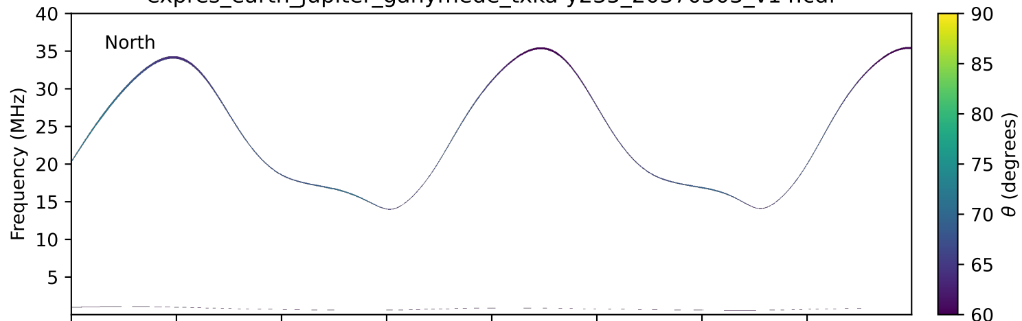
expres_earth_jupiter_ganymede_txka-y235_20370503_v14.cdf
