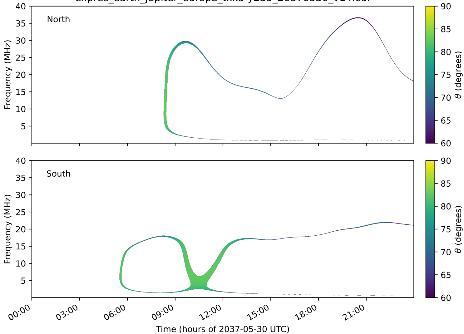
expres_earth_jupiter_europa_txka-y235_20370530_v14.cdf
