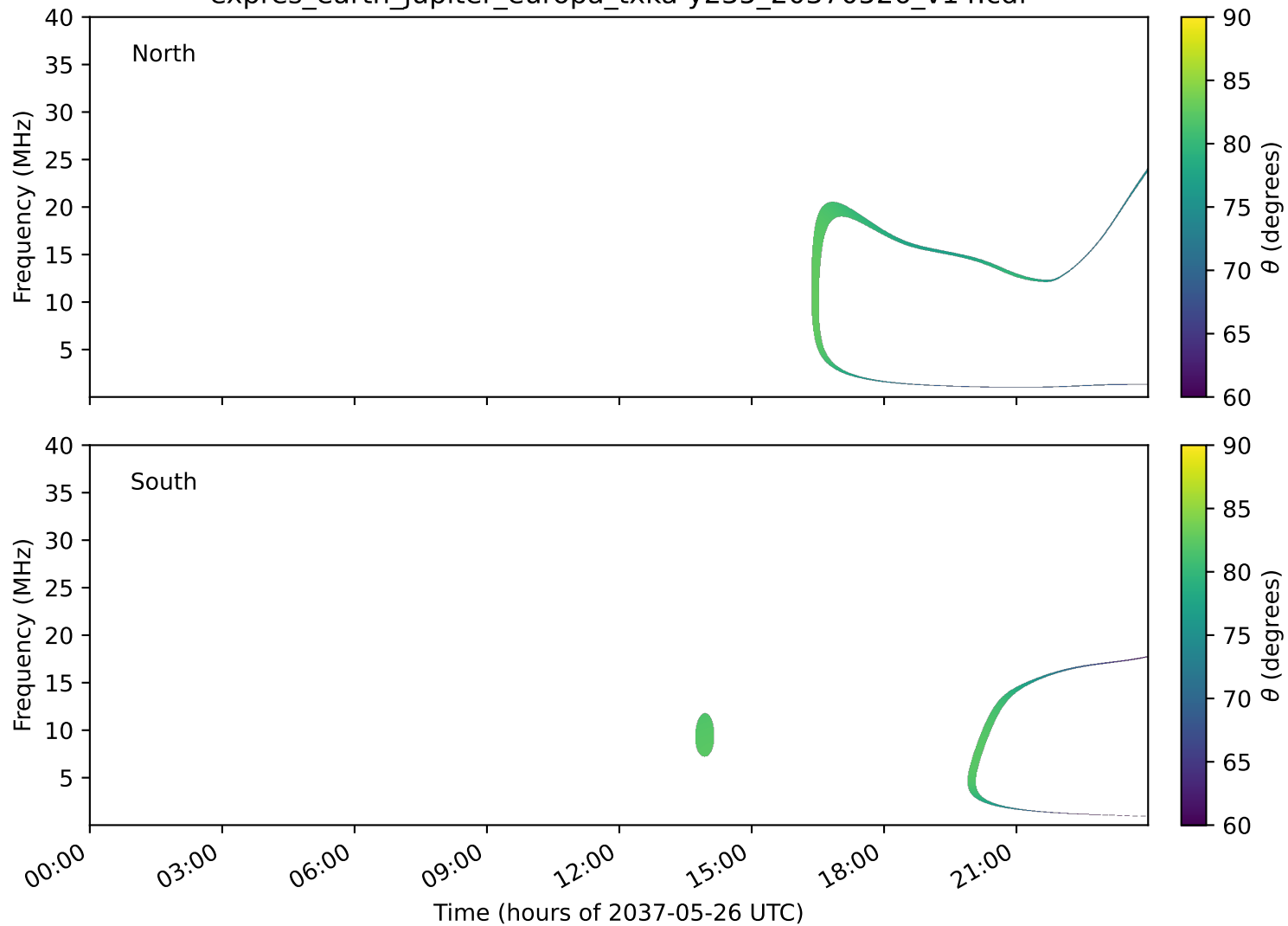
expres_earth_jupiter_europa_txka-y235_20370526_v14.cdf
