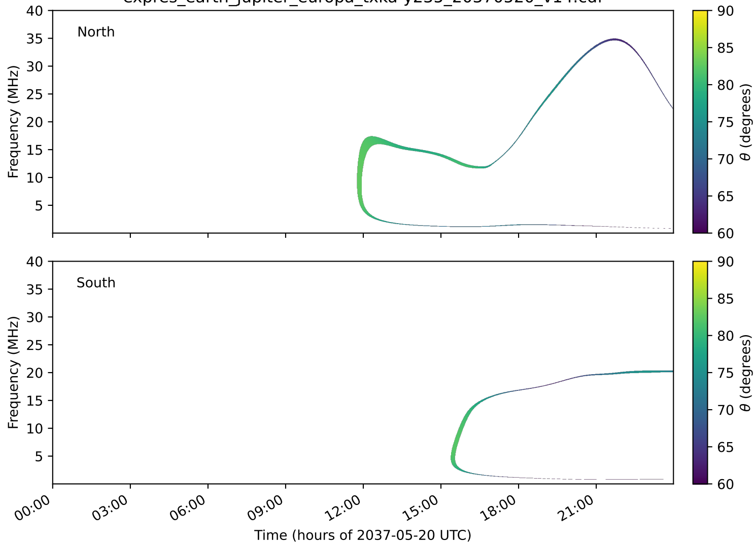
expres_earth_jupiter_europa_txka-y235_20370520_v14.cdf
