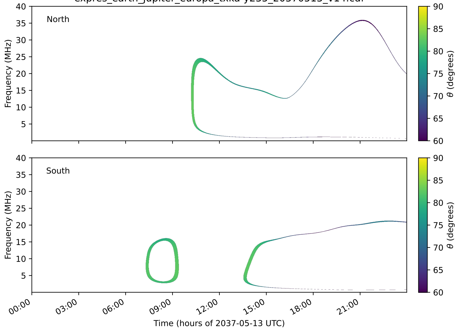
expres_earth_jupiter_europa_txka-y235_20370513_v14.cdf
