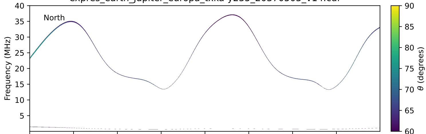
expres_earth_jupiter_europa_txka-y235_20370503_v14.cdf
