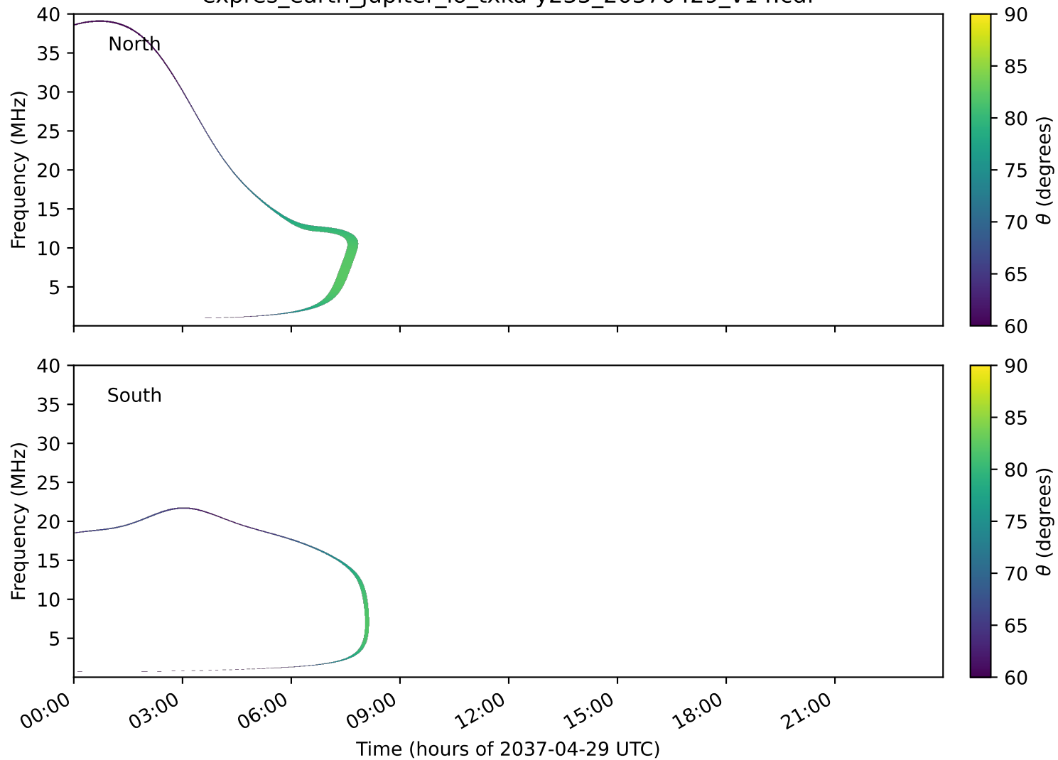
expres_earth_jupiter_io_txka-y235_20370429_v14.cdf
