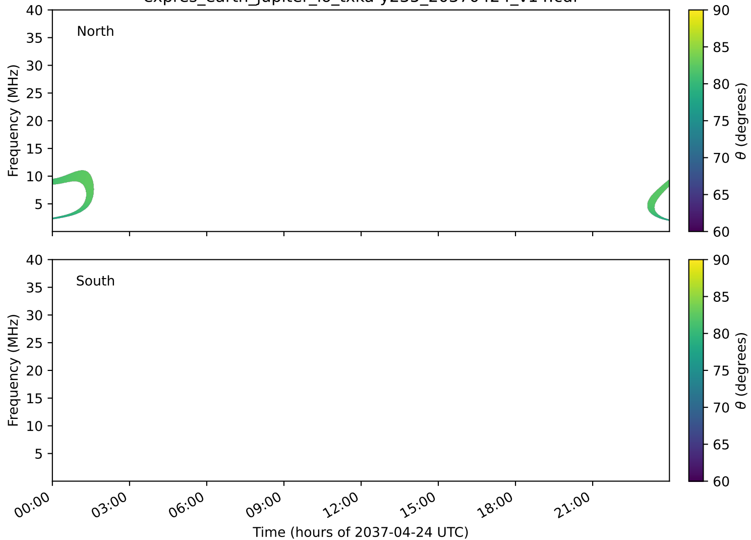
expres_earth_jupiter_io_txka-y235_20370424_v14.cdf
