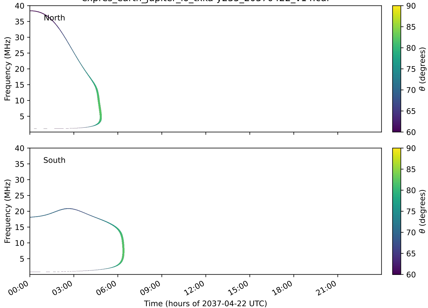
expres_earth_jupiter_io_txka-y235_20370422_v14.cdf
