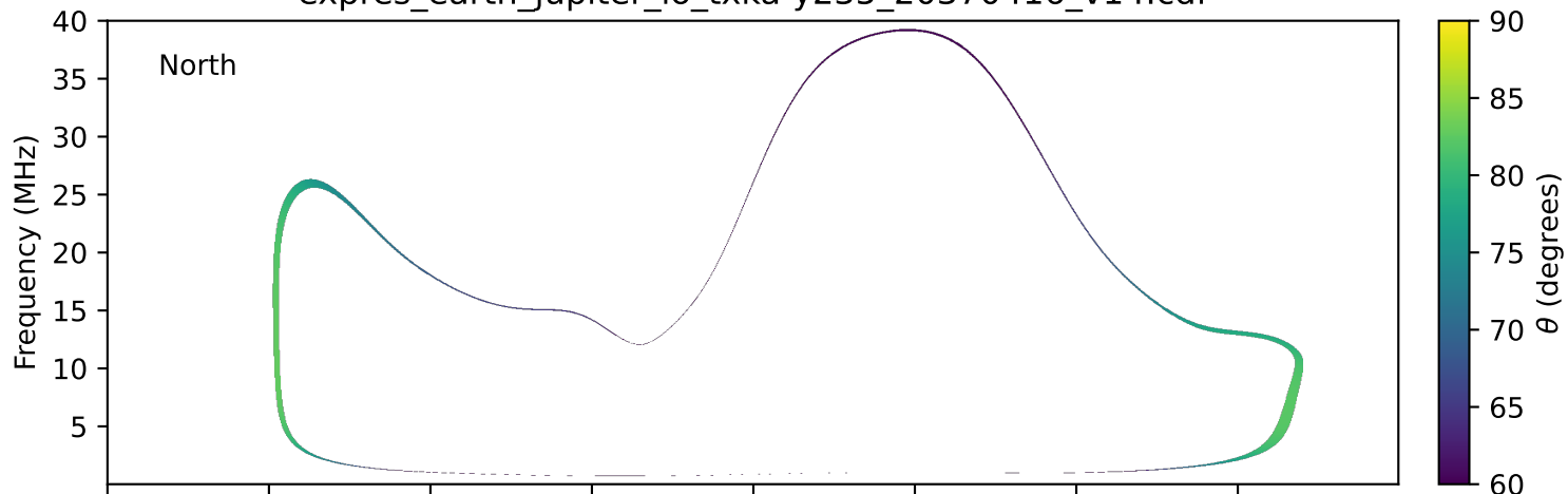
expres_earth_jupiter_io_txka-y235_20370416_v14.cdf
