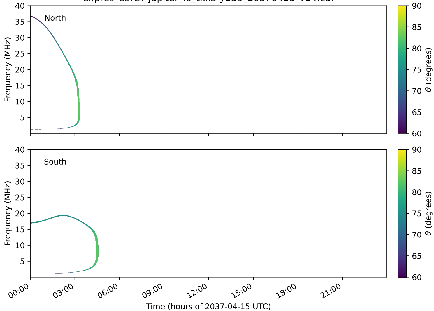
expres_earth_jupiter_io_txka-y235_20370415_v14.cdf
