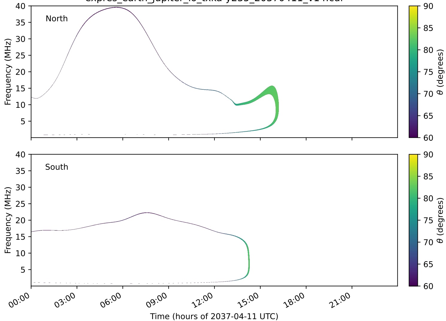
expres_earth_jupiter_io_txka-y235_20370411_v14.cdf
