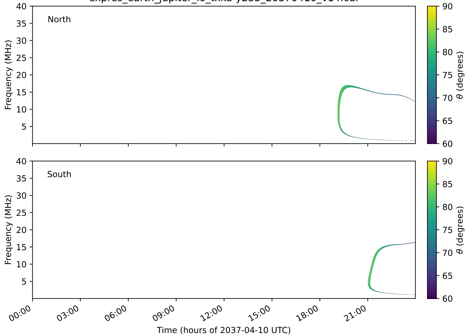
expres_earth_jupiter_io_txka-y235_20370410_v14.cdf
