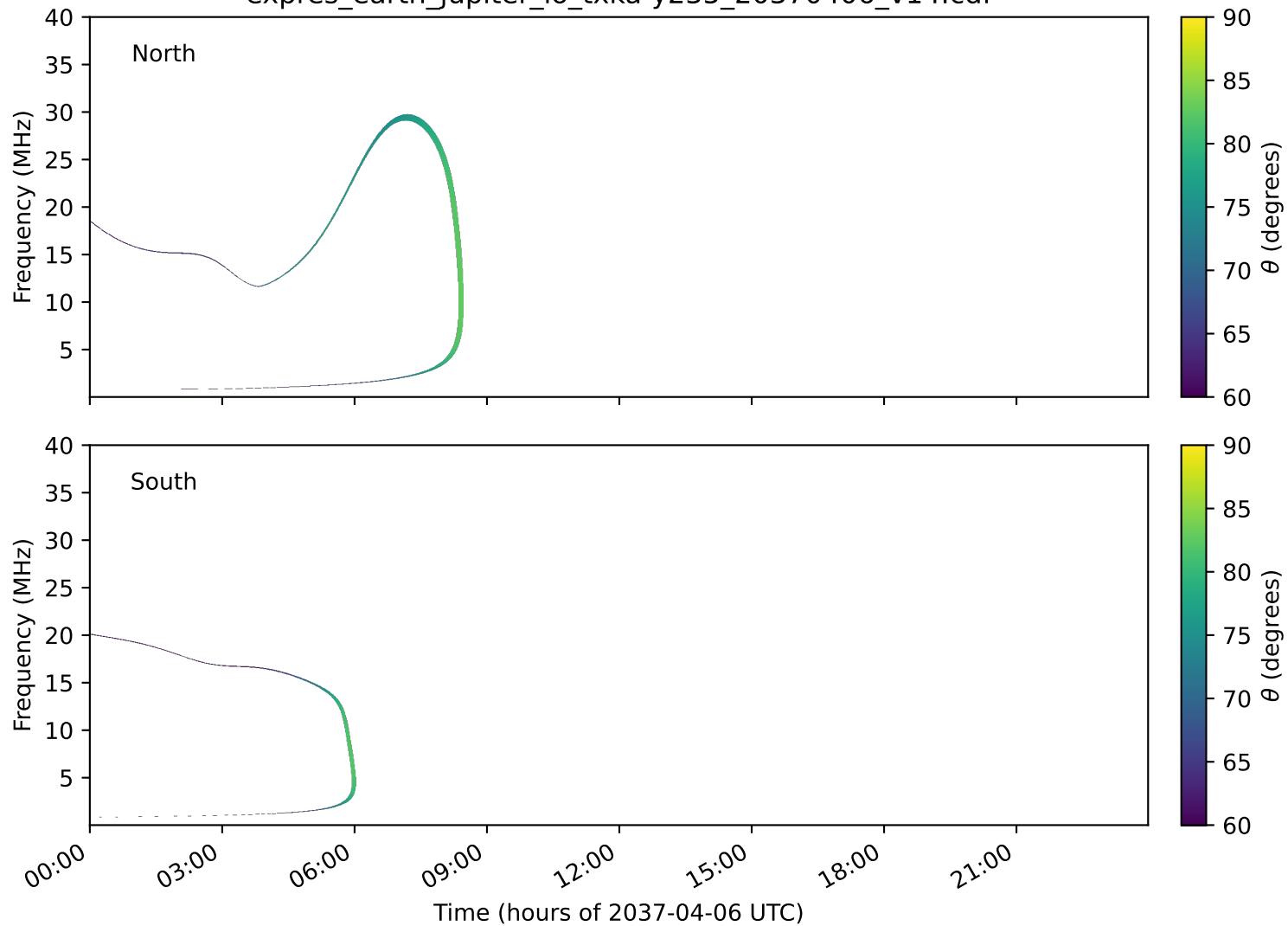
expres_earth_jupiter_io_txka-y235_20370406_v14.cdf
