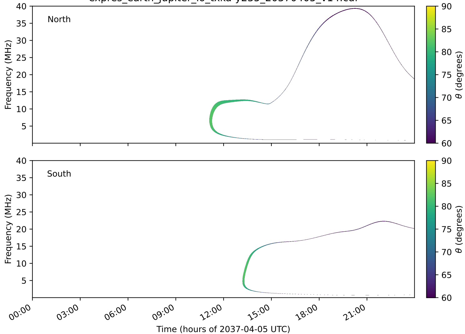
expres_earth_jupiter_io_txka-y235_20370405_v14.cdf
